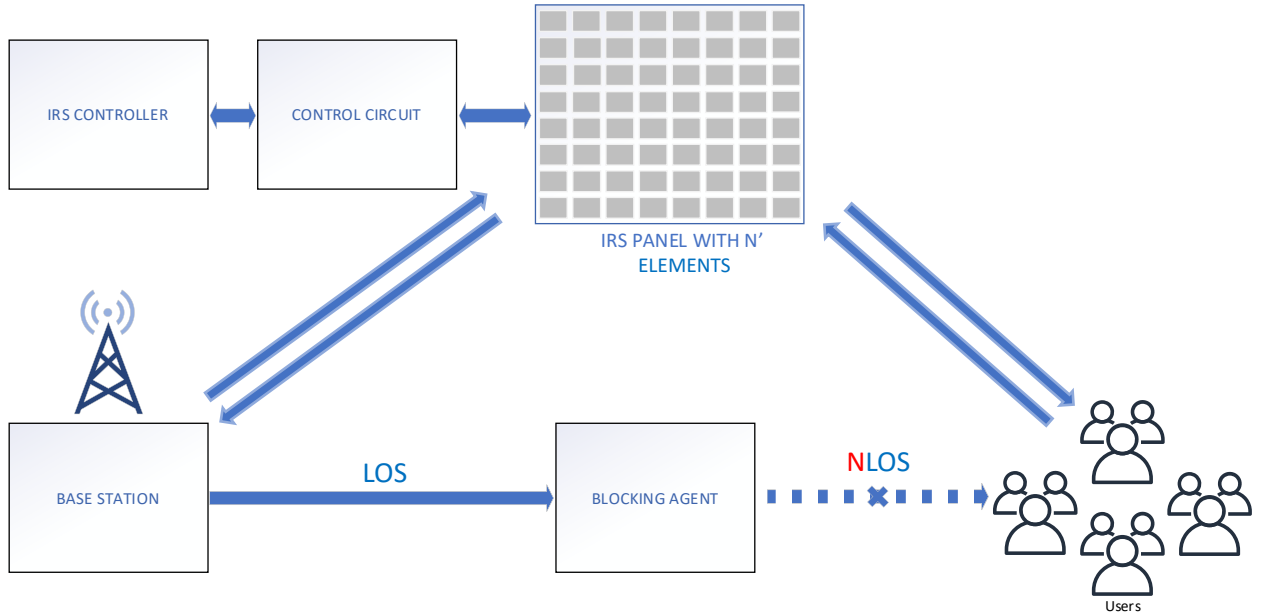
Fig 4.1 BLOCK DIAGRAM
