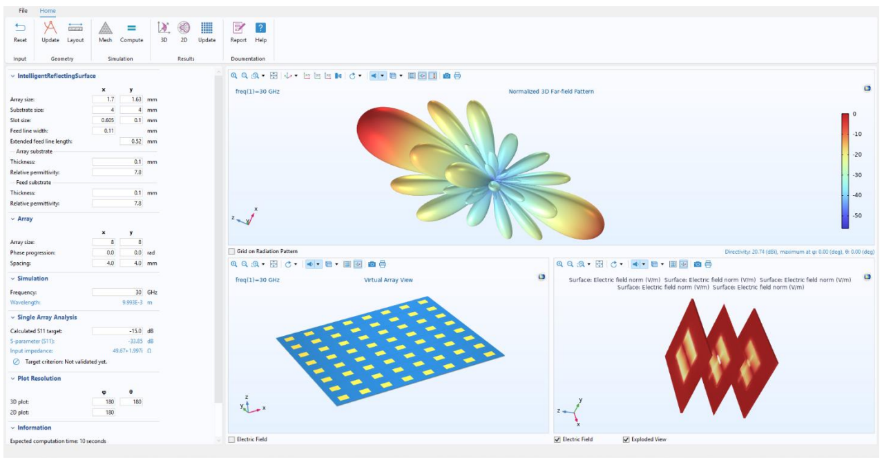
Fig 8.1.3 IRS Panel Design
